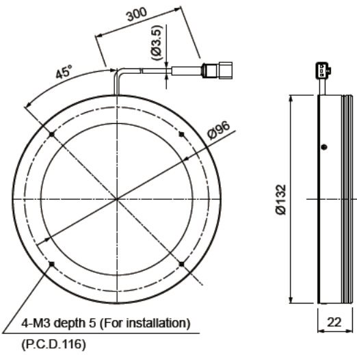
LDR2-132RD2-LA / SW2-LA / BL2-LA / GR2-LA
