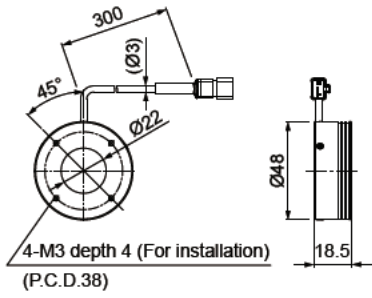
LDR2-48RD2-LA / SW2-LA / BL2-LA / GR2-LA
