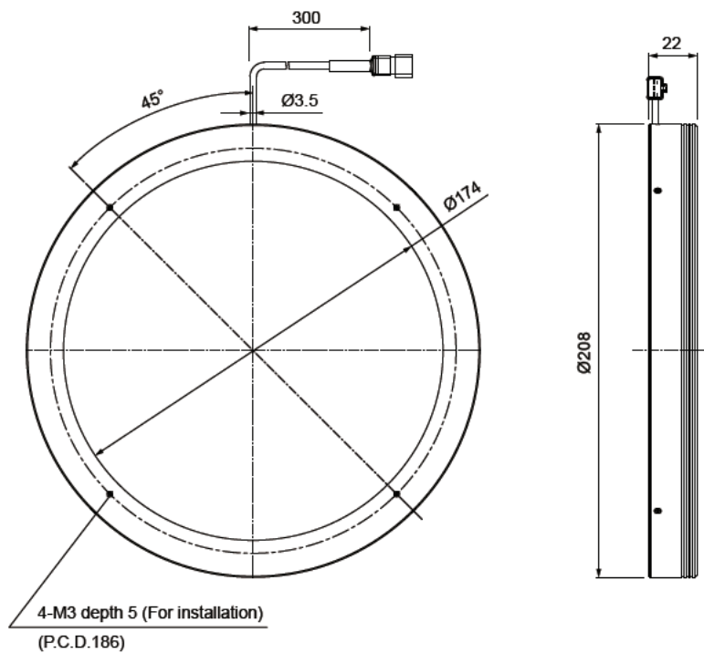
LDR2-208RD2-LA / SW2-LA / BL2-LA / GR2-LA
